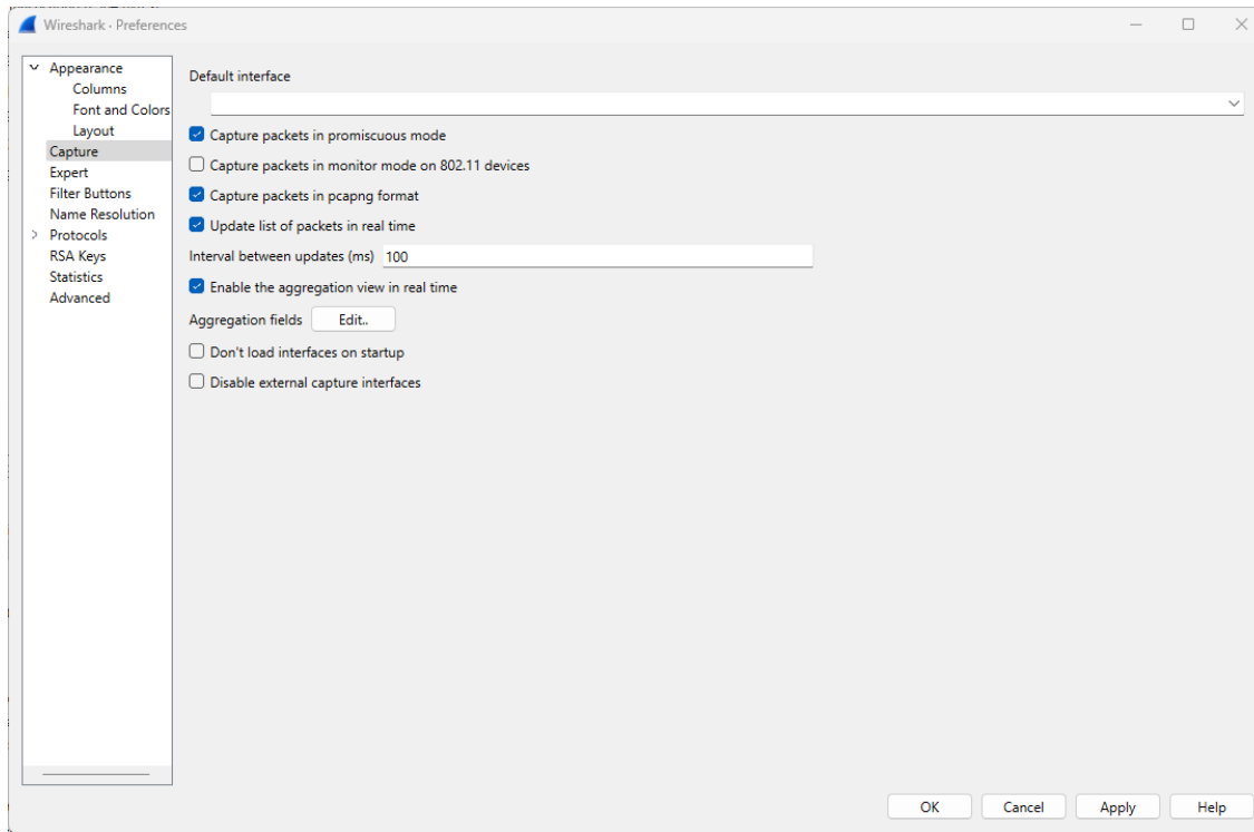
Figure 128. Capture preferences
