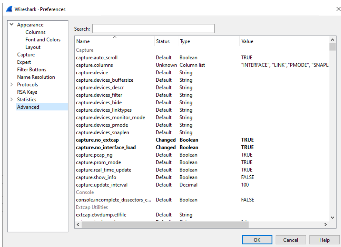
Figure 135. Advanced preferences
