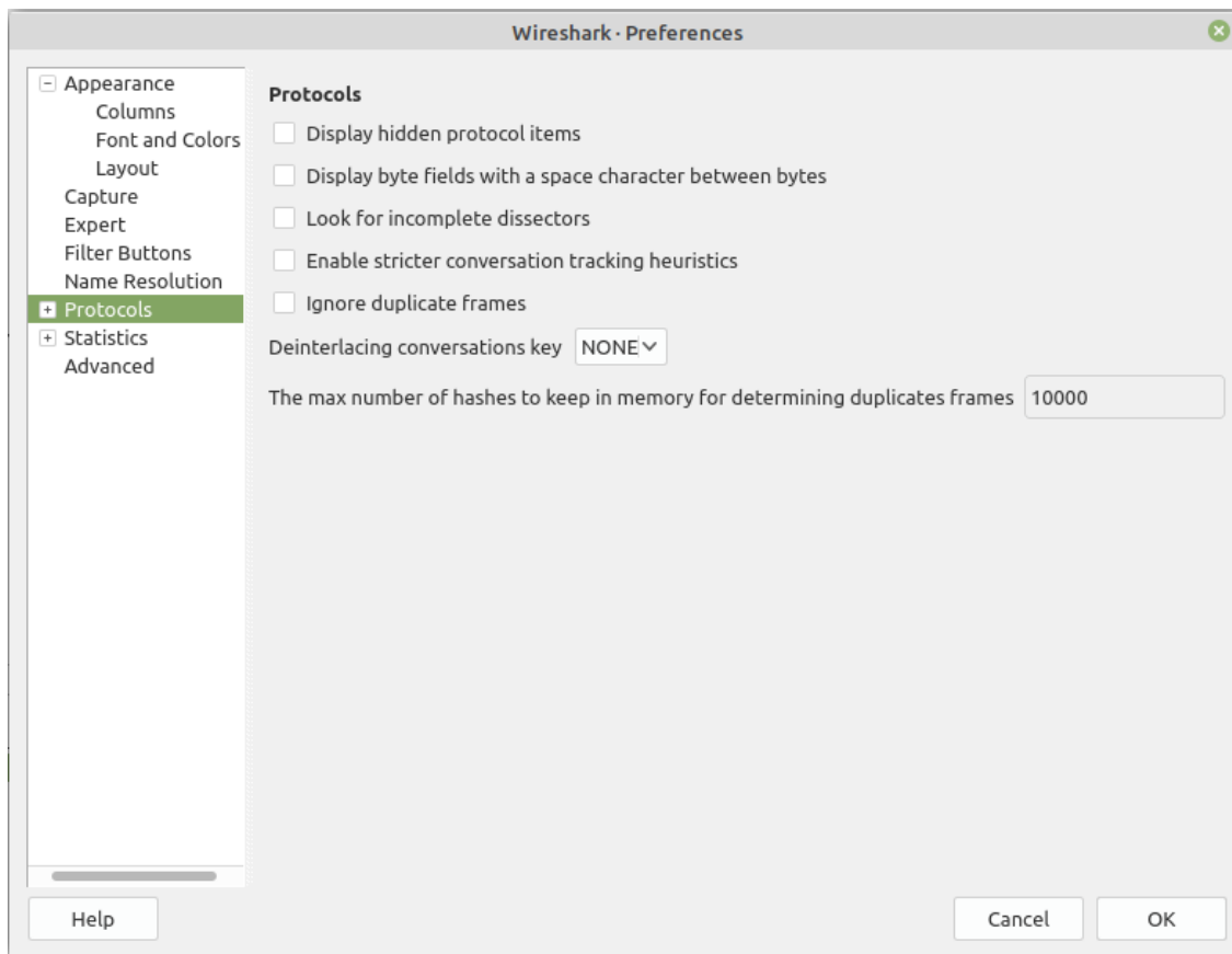
Figure 132. Protocol preferences
