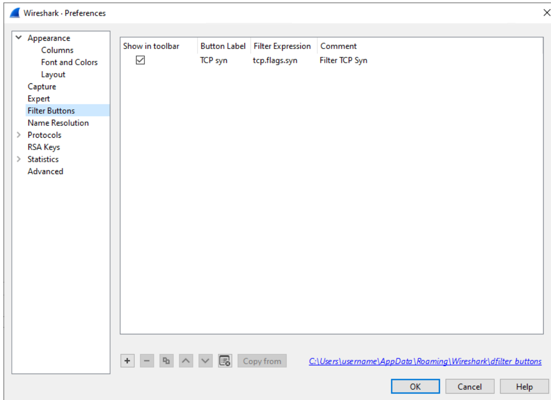
Figure 130. Filter buttons
